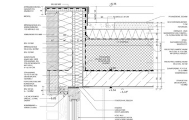
DETAILSCHNITT - ATTIKA
